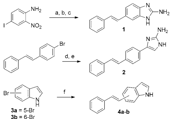
Scheme 1. Reaction conditions for the synthesis of stilbene derivatives: a) styrene, Pd(OAc) 2 , CH 3 CN, DIPEA, 80 °C, 76%; b) SnCl 2 ·2H 2 O, EtOAc, 80 °C; c) CNBr, MeOH/H 2 O (1:1), 50 °C, 91% (over two steps); d) imidazo[1,2- a ]pyrimidine hydrobromide, Pd(OAc) 2 , PPh 3 , Cs 2 CO 3 , 1,4-dioxane, 100 °C, 82%; e) 20% N 2 H 4 /EtOH, 105 °C, 84%; f) styrene, Pd(OAc) 2 , P( o -tolyl) 3 , NEt 3 , 100 °C, 73–76%. DIPEA = N,N -diisopropylethylamine.
